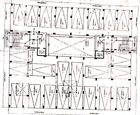
GROUND FLOOR PLAN OF TOWER 4 SCALE: 1 : 100
